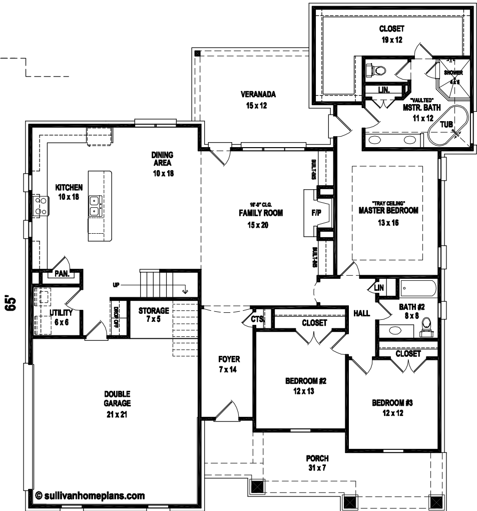
FIRST LEVEL FLOOR PLAN
